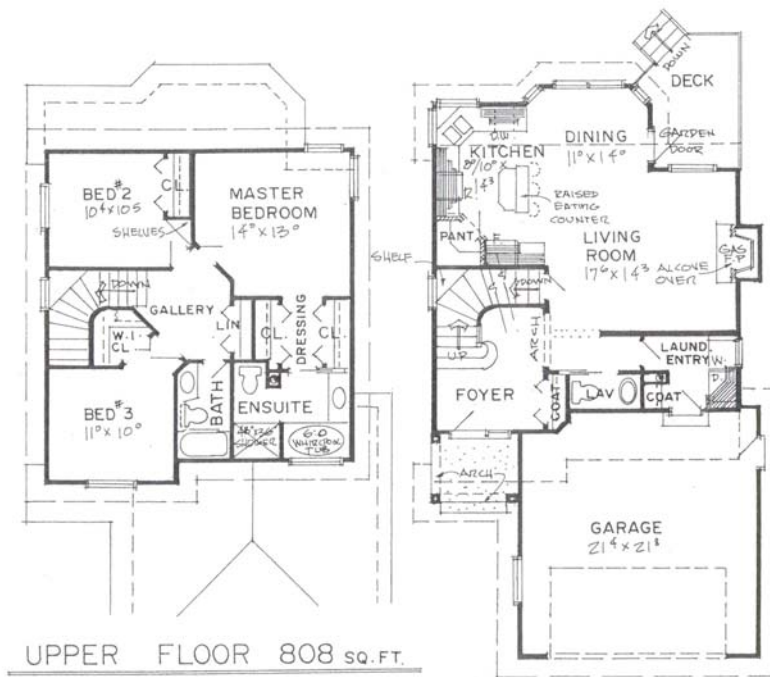
1595 SQ.FT. TOTAL
