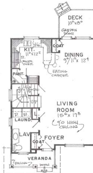
MAIN FLOOR 772 SQ. FT.
